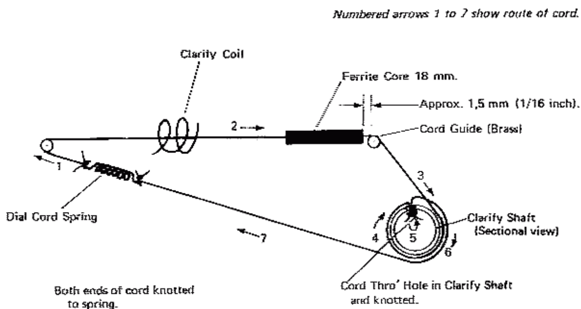
FRONT VIEW OF CLARIFY MECHANISM SHOWN WITH CLARIFY SHAFT FULLY CLOCKWISE.
